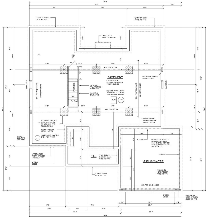
BASEMENT & FOUNDATION PLAN
